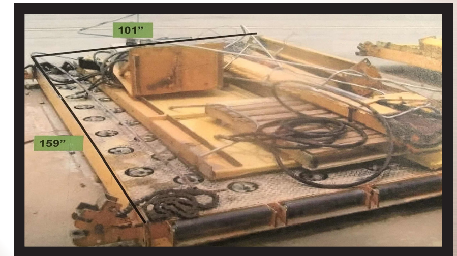
Dismantled ULD Lift
